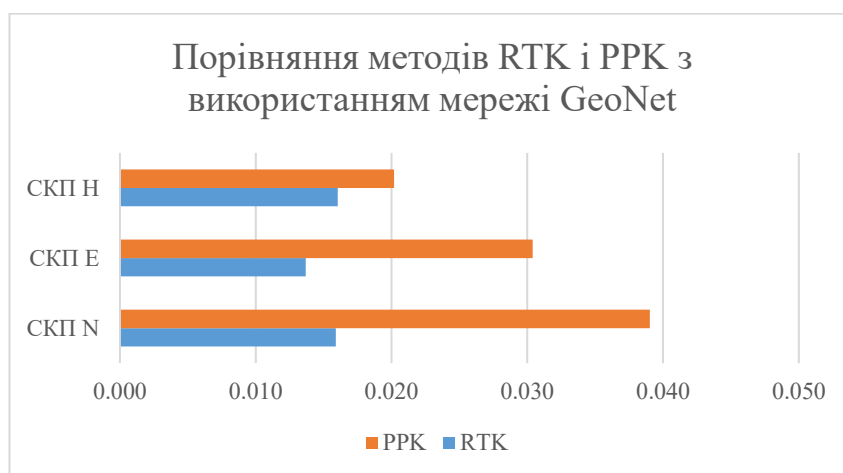
Diagram 3. Comparison of the total RSM in RTK (GeoNet) and PPK (GeoNet) modes
