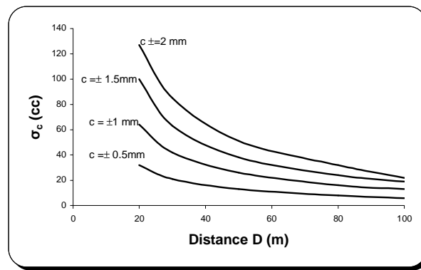
Figure 2 - The error in the angle measurement \sigma_c relative to the distance D and the centering error c .
