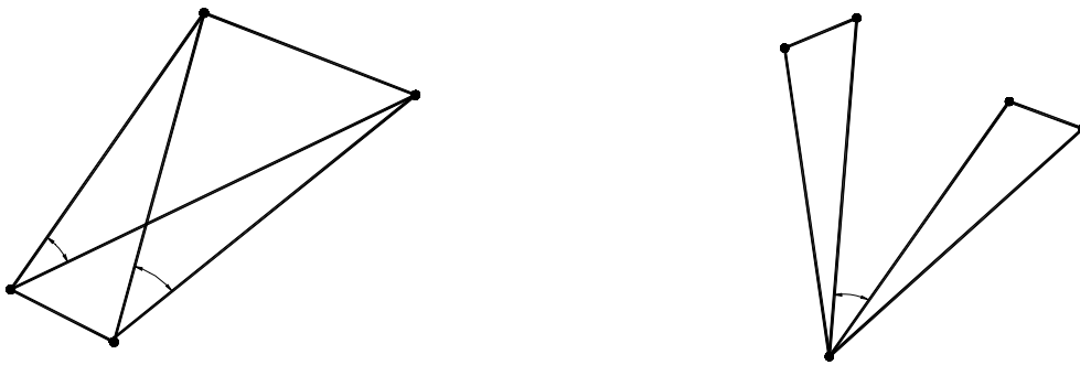
Figure 1a- The centering error of the instrument Figure 1b- The centering error of the targets
