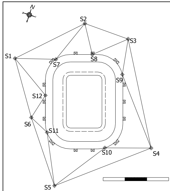
Figure 4 - The control network of the stadium.
