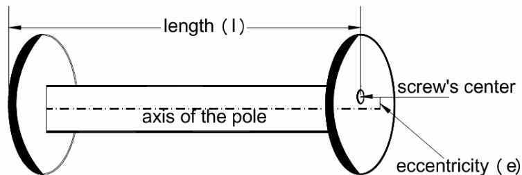
Figure 3 - The geometric characteristics of the pole.
